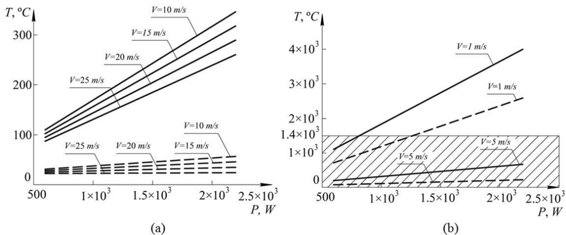
Fig. 2. Changes in the particle temperature depending on the laser radiation power and particle velocity: (a) - V = 10-25 m/s, (b) - V = 1-10 m/s. Solid lines - irradiated side of particle, dash lines - nonirradiated side of particle.
